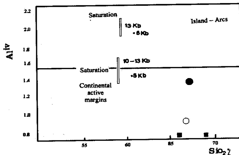
Fig. 6 Limit of [Al^{IV}] = 1.5 allows which amphiboles and therefore magmas of Island arcs are being recognized from amphiboles and magmas of continental active margins (the case in the study area) [18]. Open bars showing range of variations of syntetic amphiboles under, pressures of 5 kbar [14].
