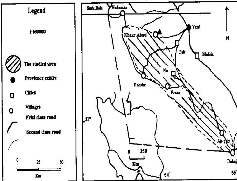
Fig. 1 Geographical position of granitoid of Kheyr-Abad (NW, Taft, central Iran). ▲: Kheyr-Abad
