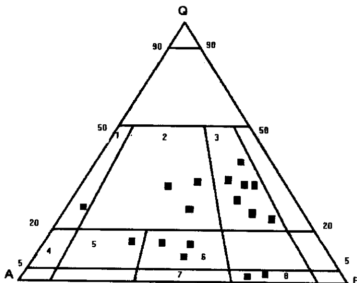
Fig 2 Streckeisen diagram (1982) Showing plot of igneous rocks of the studied area. 1- Alkali feldspar granite 2- Granite 3- Granodiorite 4- Quartz-syenite 5- Quartz-monzonite 6- Monzo-diorite 7- Tonalite 8- Syenite
