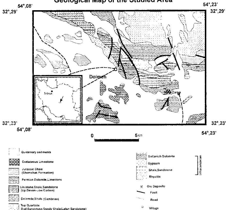
Geological Map of the Studied Area
