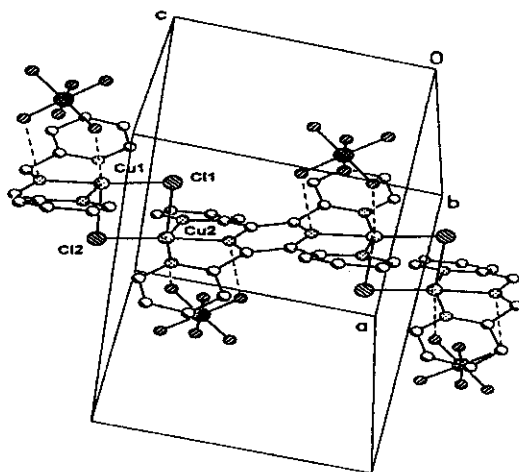
Figure 2 Cell drawing of the complex, [\{\text{CuCl}\}_2(\mu\text{-tppz})](\text{PF}_6)_2 . Selected bond lengths (Å) and bond angles (deg): Cu2-Cl2, 2.2431(12); Cu1-Cl2, 2.7196(13); Cu1-Cl2-Cu2, 83.20(4); Cl1-Cu1-Cl2, 96.80(4).
