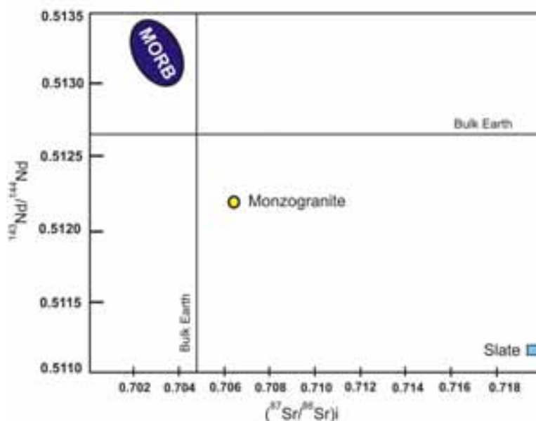
Figure 11. Plot of (^{87}\text{Sr}/^{86}\text{Sr})_i versus ^{143}\text{Nd}/^{144}\text{Nd} .
