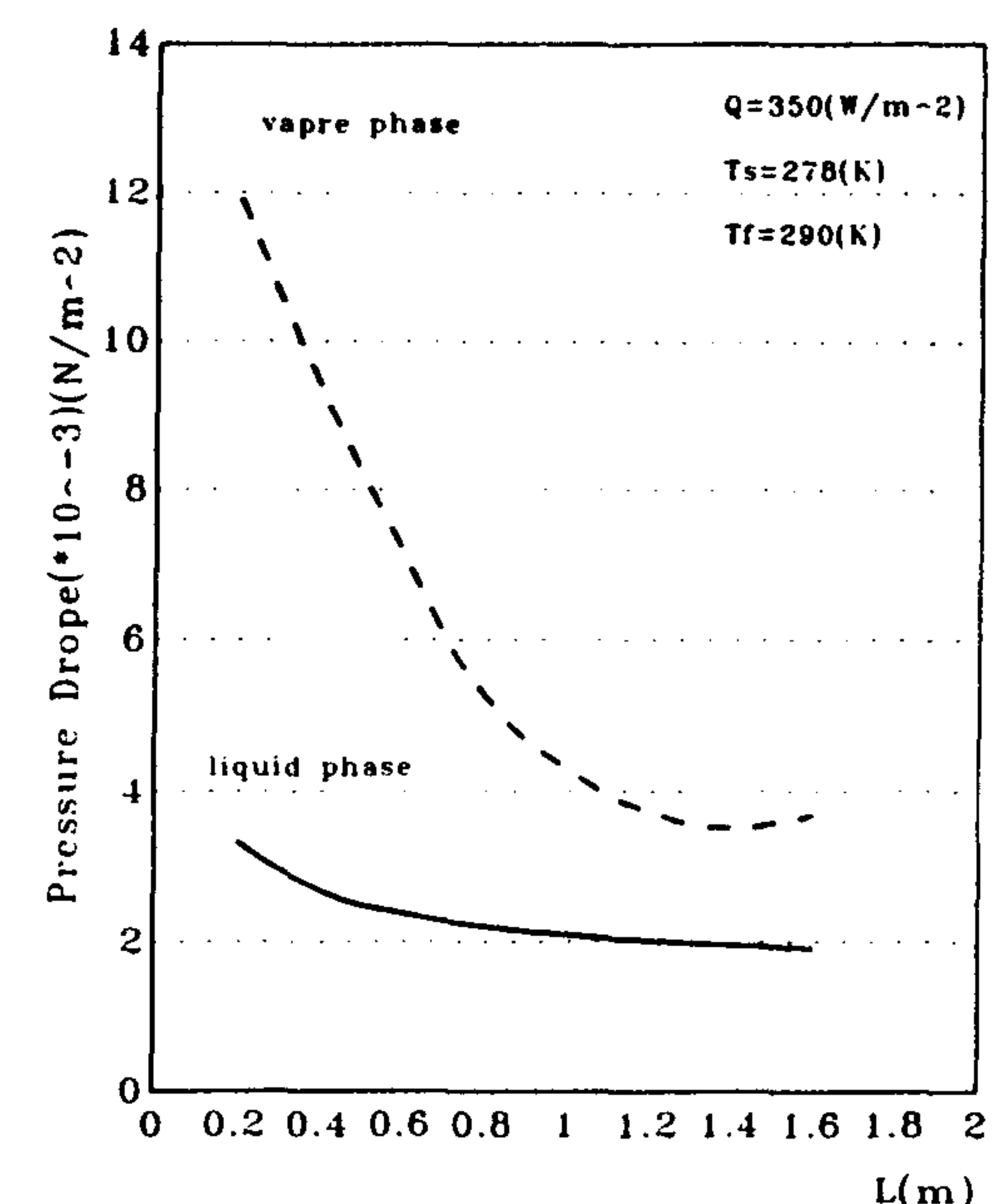
PRESSURE DROP CHANGINGS OF LIQUID & VAPORE PHASE AT DIFF. LENGTH OF THE HEAT PIPE.
