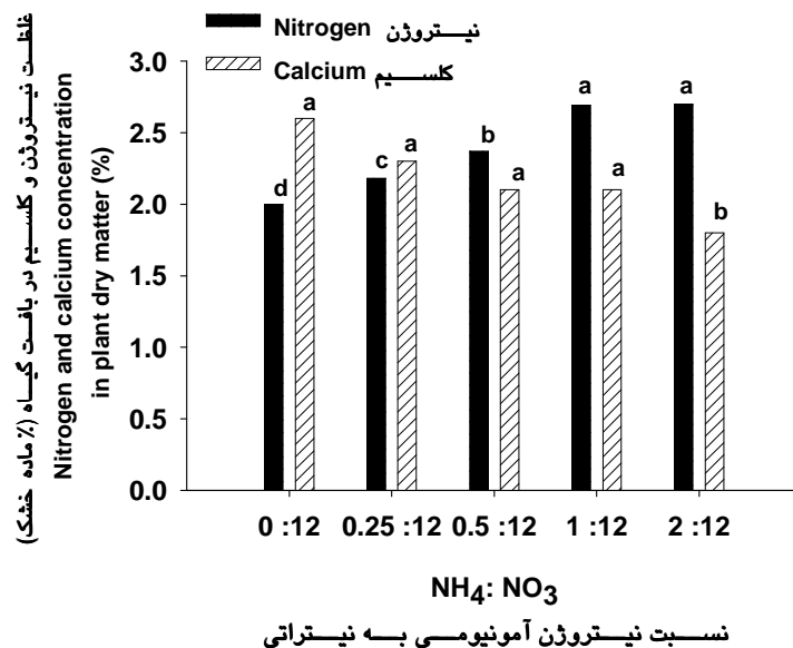
Fig. 3. N and Ca concentrations of rose plants affected by different ratios of \text{NH}_4^+:\text{NO}_3^- in nutrient solutions. Bars with different letters are significantly different ( P < 0.05 , DMRT).
