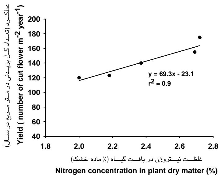
Fig. 4. correlation between rose cut flowers yield and plant N concentration as affected by different ratio of \text{NH}_4^+:\text{NO}_3^- in nutrient solutions.
