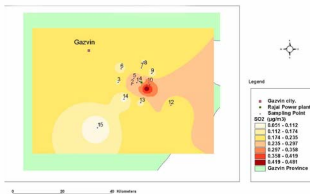
Concentration of SO 2 around Rajaei
