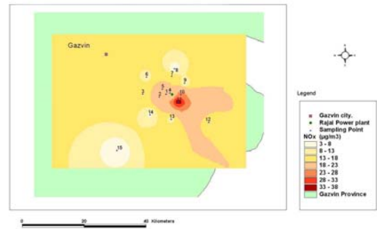
Concentration of NO x around Rajaei power
