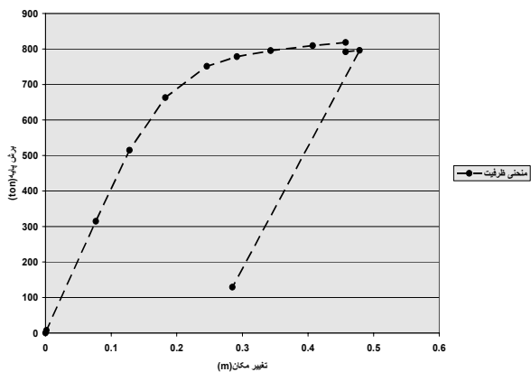
S Pushover : ( )
