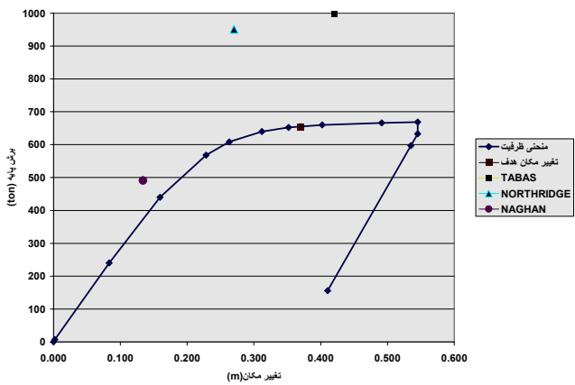
S Pushover : ( )
