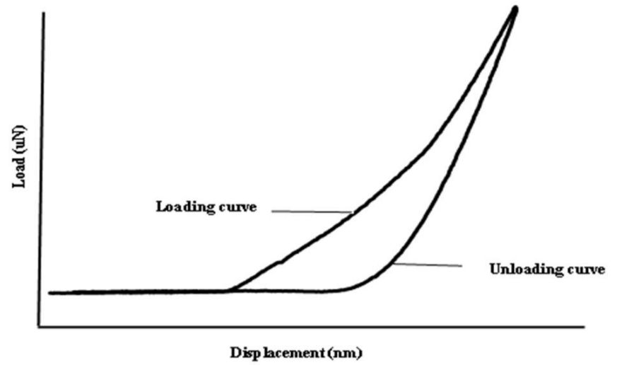
Fig. 5 Schematic curve of loading-unloading PLA neat by using nanindentation
