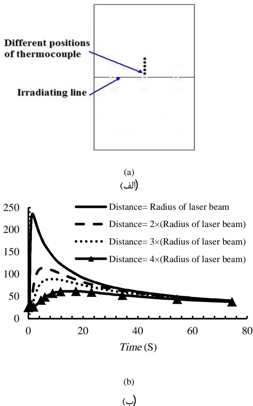
Fig. 8 Allowable distance between adjacent irradiating lines, a- Schematic of various positions of the thermocouple from irradiating line, b- The diagram of transferred heat to adjacent points with different displacements related to irradiating line
