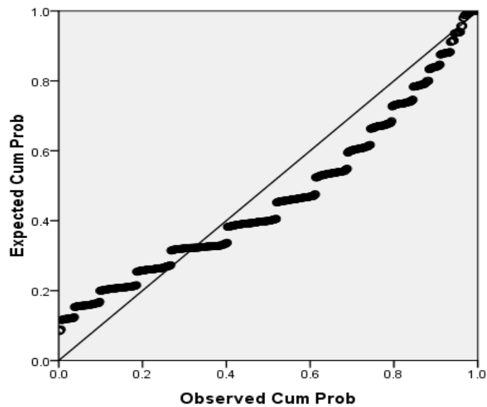
Normal P-P Plot of Standardized Residual
